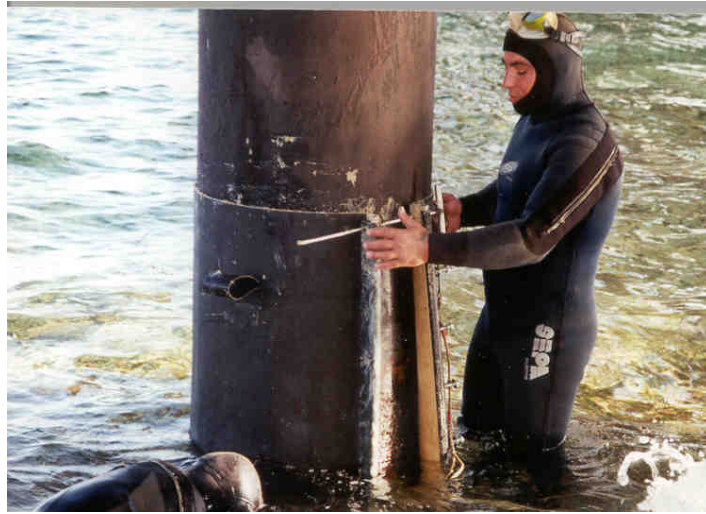
Fitting line up rod into flanges Note sealing faces and grab handle clearly visible
